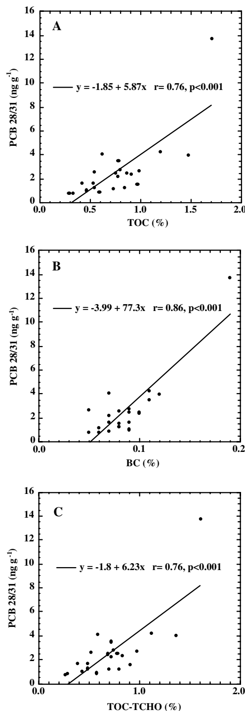
Fig. 5. Relationships between concentrations of (A) PCBs 28/31 and organic carbon (TOC); (B) PCBs 28/31 and BC; (C) PCBs 28/31 and TOC-TCHO in the sediments of the Danshui River.
