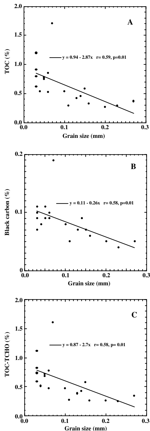
Fig. 2. Relationships between (A) grain size and TOC; (B) grain size and black carbon, BC (B); and (C) grain size and TOC-TCHO concentrations.
