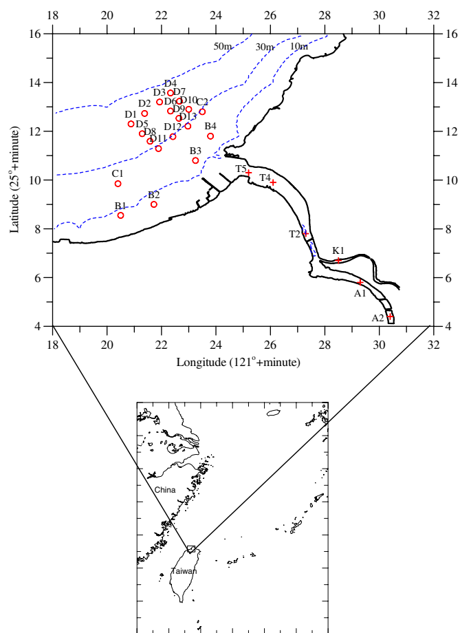
Fig. 1. Sediment sampling stations in the Danshui River and nearby coastal zone, Taiwan.
