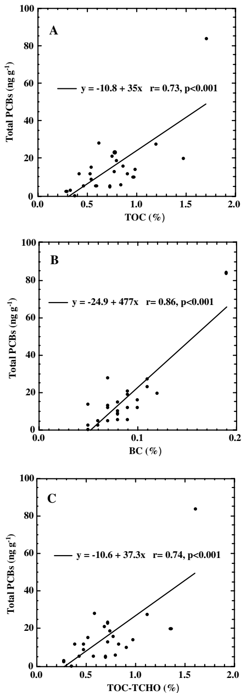
Fig. 3. Relationships between (A) total PCBs and TOC; (B) total PCBs and black carbon; and (C) total PCBs and TOC-TCHO concentrations.
