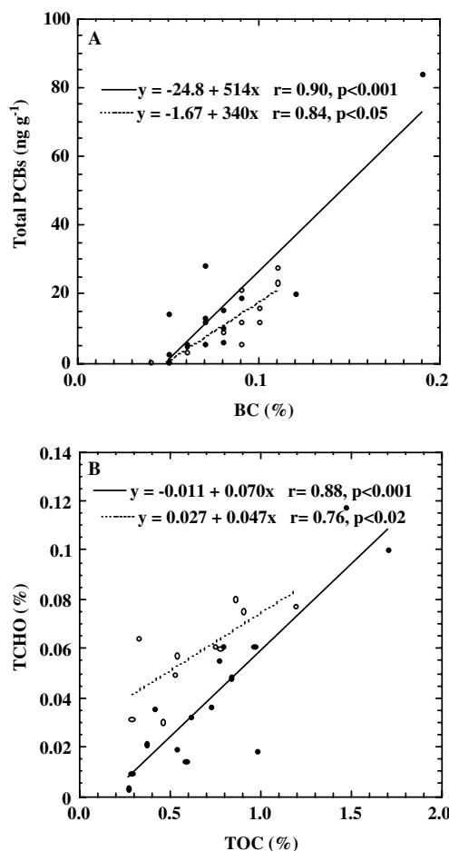
Fig. 4. Relationships between concentrations of (A) total PCBs and BC; (B) TCHO and TOC. Solid symbols denote shallow water group (<30 m) and open symbols denote deep water group (>30 m).
