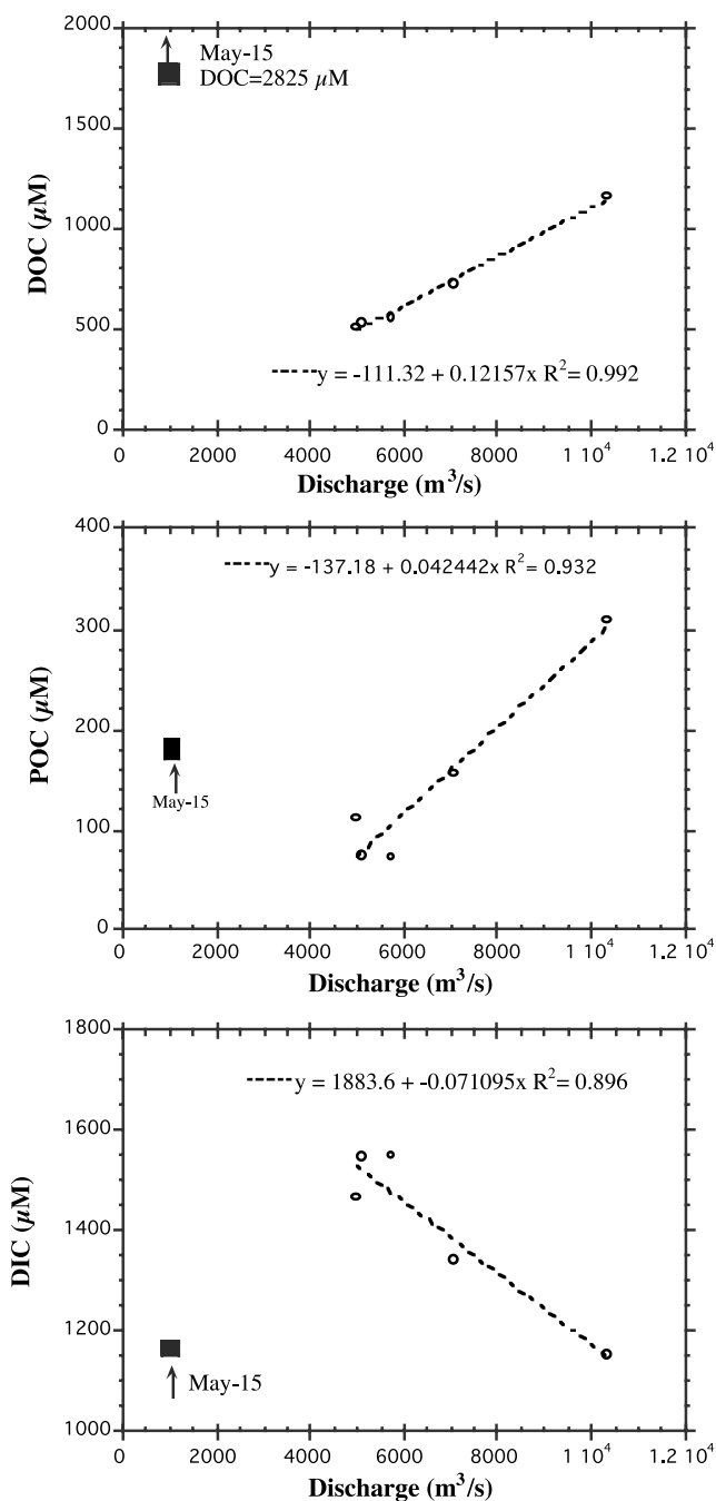
Figure 3. Relationship between river discharge (m 3 /s) and dissolved organic carbon (DOC), particulate organic carbon (POC), and dissolved inorganic carbon (DIC) concentrations.
