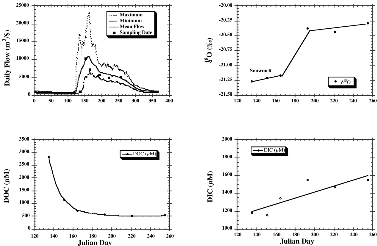
Figure 2. Temporal variations of daily freshwater discharge ( \text{m}^3/\text{s} ), dissolved organic carbon (DOC, <0.45 \mu\text{m} ) and dissolved inorganic carbon (DIC) concentrations (all in \mu\text{M} ), and stable oxygen isotope ( \delta^{18}\text{O} ) composition in Yukon River waters. Discharge data are from 1976 to 2000 with maximal, minimal, and mean values (from U.S. Geological Survey at http://www.uags.gov ). Also shown on this plot are the sampling dates (solid points) with their corresponding instantaneous freshwater discharge in 2002.
