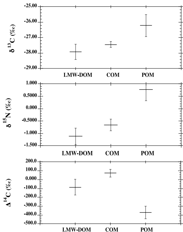
Figure 5. Distributions of stable isotope ( \delta^{13}\text{C} and \delta^{15}\text{N} ) and \Delta^{14}\text{C} values among dissolved, colloidal, and particulate organic matter showing the heterogeneity of riverine organic matter.
