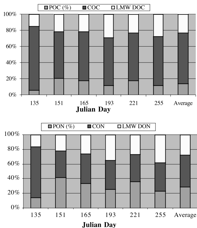
Figure 4. Partitioning of organic C and N among low-molecular-weight dissolved (LMW, <1 kDa), colloidal, and particulate phases in Yukon River waters and its temporal variation from May to September 2002.
