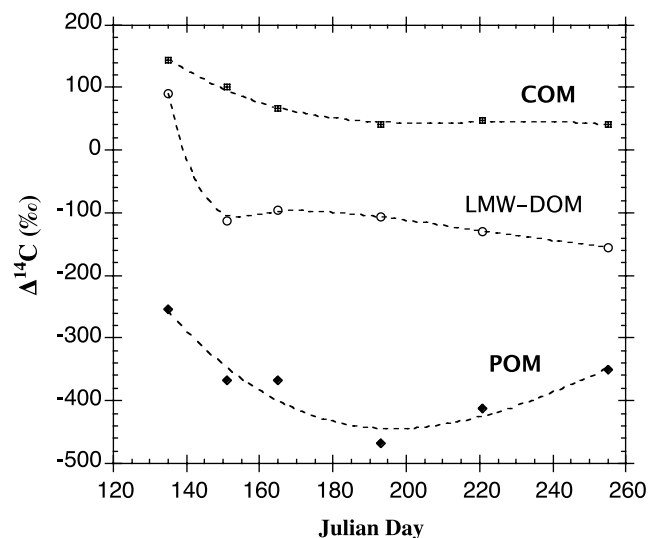
Figure 6. Variations of \Delta^{14}\text{C} values (‰) of POM, COM and LMW-DOM with sampling date. Notice the general decrease in \Delta^{14}\text{C} values (increase in ^{14}\text{C} age) from COM to LMW-DOM to POM, and the decreasing trend from snowmelt to river ice-open season.
